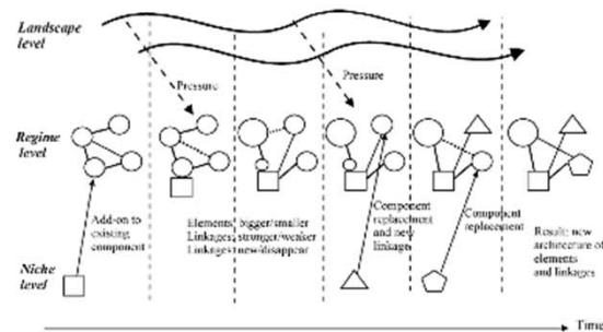
Fig. 10. Reconfiguration pathway.
