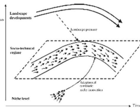
Fig. 5. Transformation pathway.
